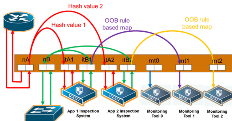
Figure 92 Out-of-Band Rule-Based Maps
