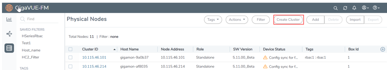
Figure 11 Create Cluster
