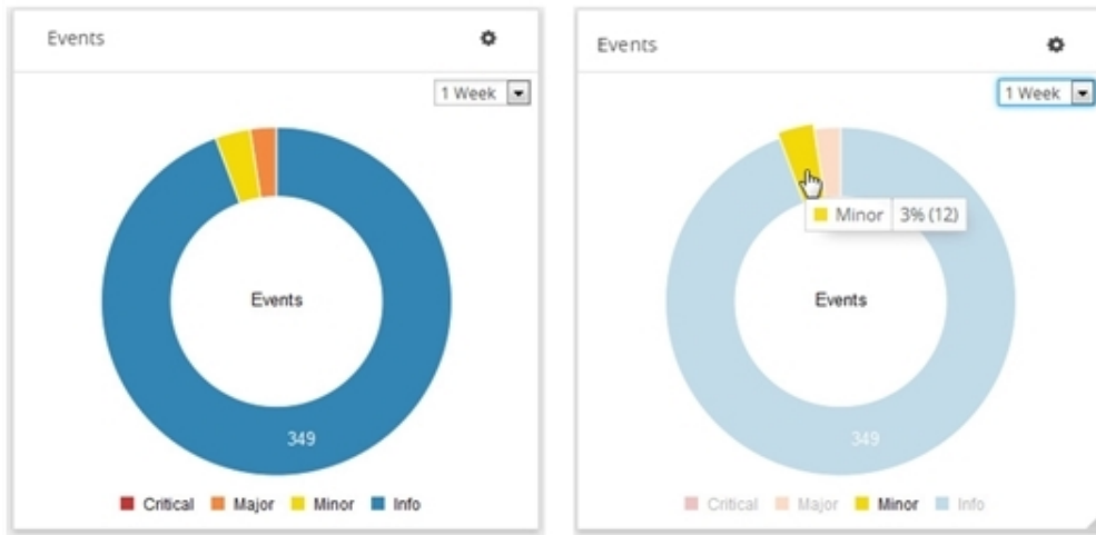
Figure 44 Events Widget
