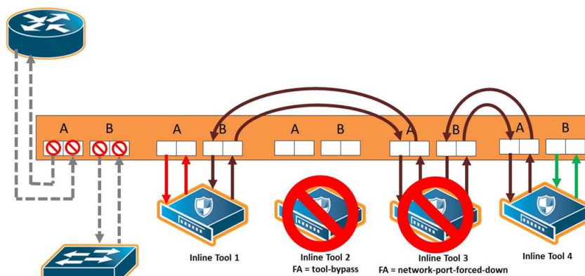
Figure 87 Inline Tool Series Local Failover of Two Tools
