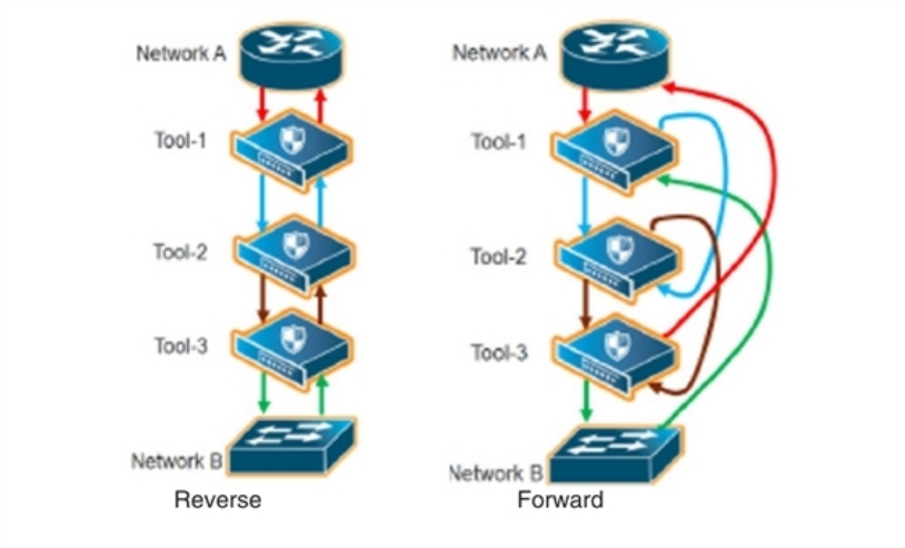
Figure 88 Inline Tool Series Per-Direction Order: Simplified Reverse and Forward
