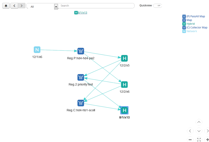
Figure 43 Map Selected
