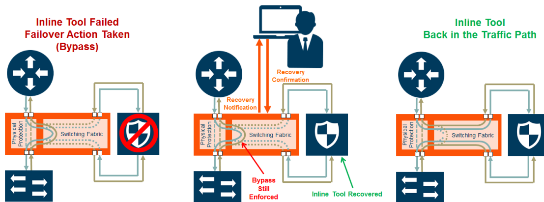
Figure 71 Automatic and Manual Inline Tool Recovery from Failover
