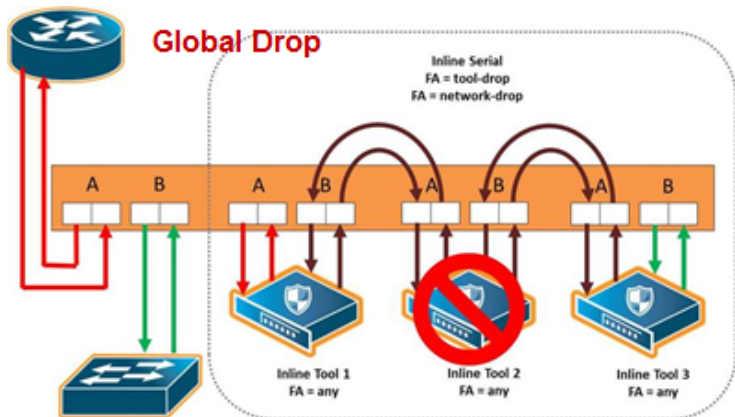
Figure 81 Inline Tool Series Global Drop Failover Action
