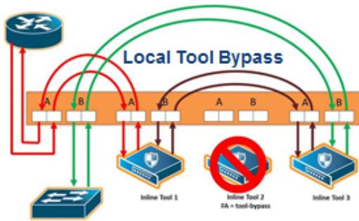
Figure 82 Inline Tool Series Local Tool Bypass Failover Action
