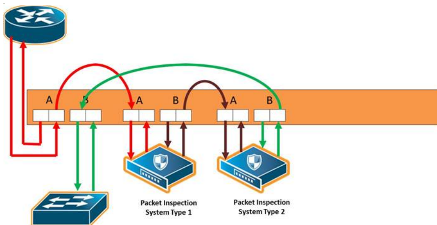
Figure 60 Inline Tool Series
