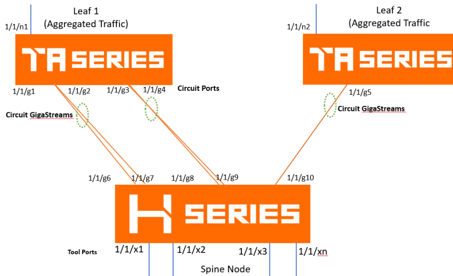
Figure 109 Circuit GigaStreams in Fabric Maps
