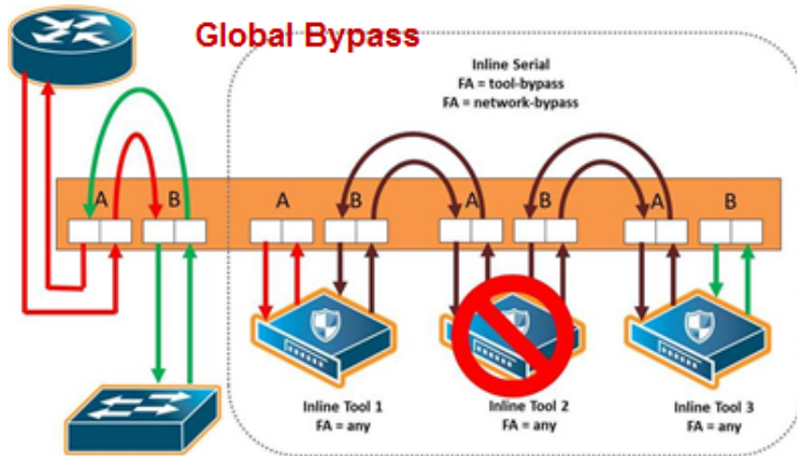
Figure 79 Inline Tool Series Global Bypass Failover Action
