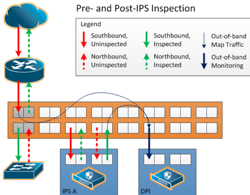
Figure 63 Out-of-Band Arrangement
