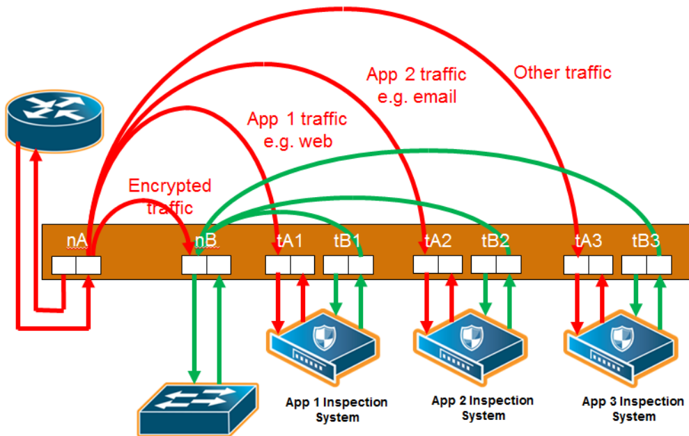
Figure 62 Inline Flow Mapping® Based Traffic Distribution
