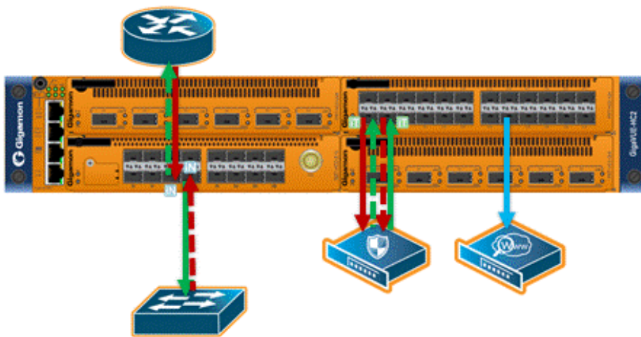
Figure 99 Logical Bypass Without Bypass Combo Module
