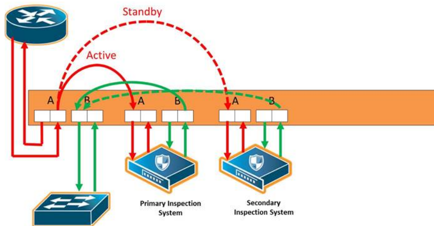
Figure 74 Inline Tool Group With Spare, Redundant 1+1 Scenario
