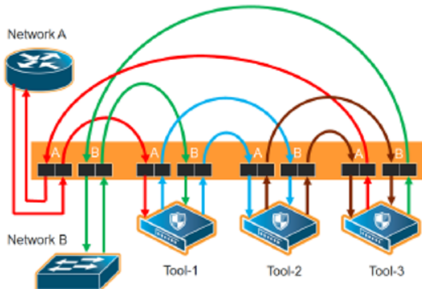
Figure 90 Inline Tool Series Per-Direction: Forward
