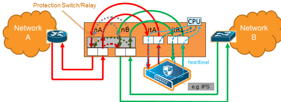
Figure 57 Physical Bypass Protection
