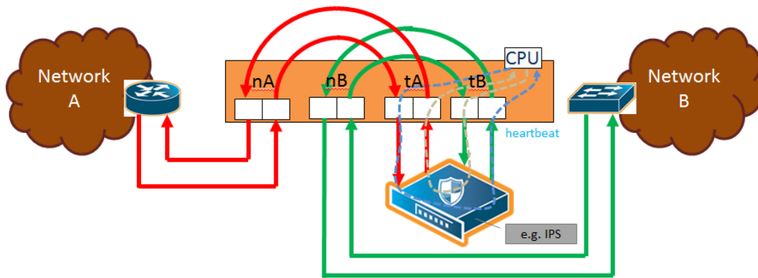
Figure 67 Traffic Path of To-Inline-Tool
