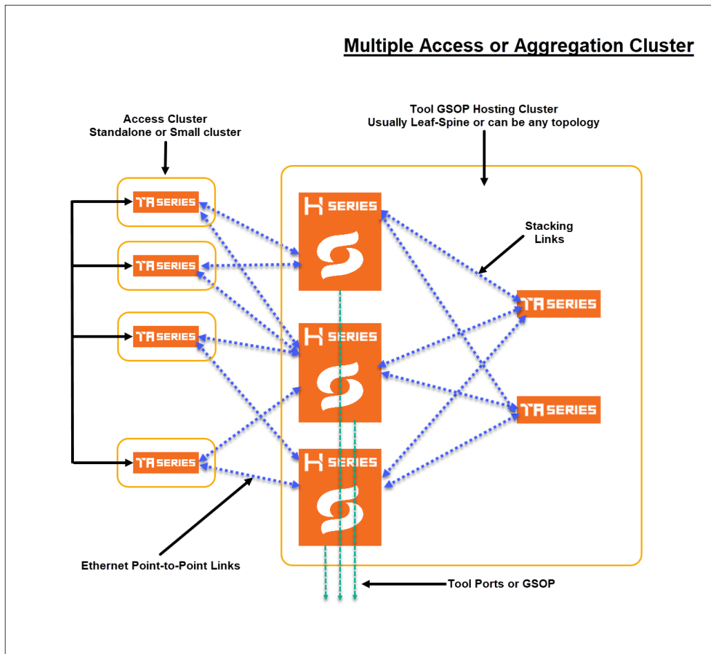
Figure 108 Multiple Access Clusters
