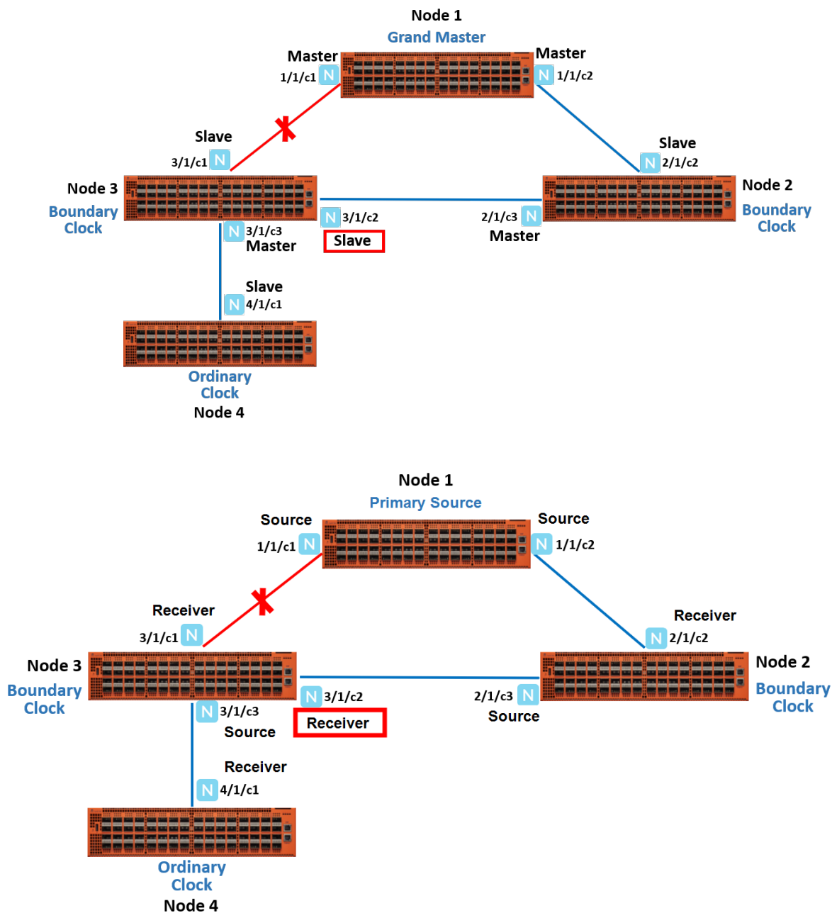
Figure 102 PTP State Transition
