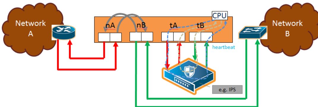
Figure 65 Traffic Path of Bypass
