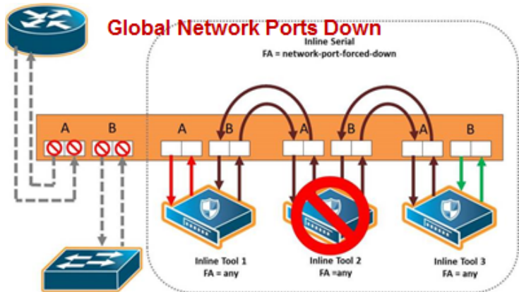
Figure 80 Inline Tool Series Global Network Ports Forced Down Failover Action
