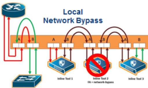
Figure 84 Inline Tool Series Local Network Bypass Failover Action
