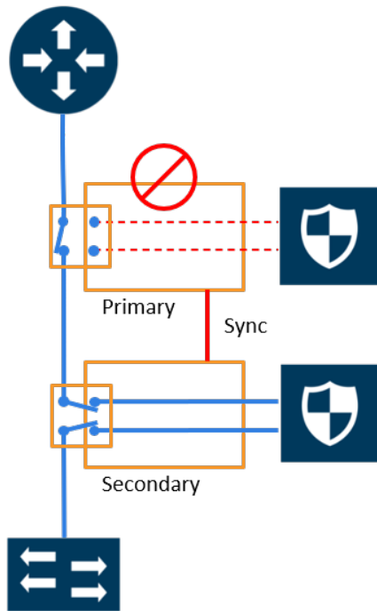
Figure 96 Traffic Flows Through Node with Secondary Role after Primary is Lost
