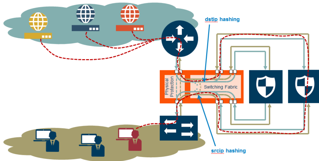
Figure 76 Asymmetrical Hashing
