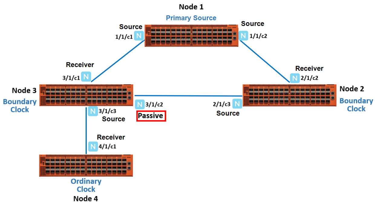
Figure 101 PTP Deployment
