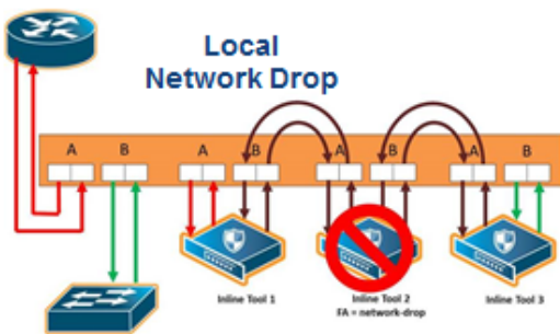
Figure 85 Inline Tool Series Local Network Drop Failover Action
