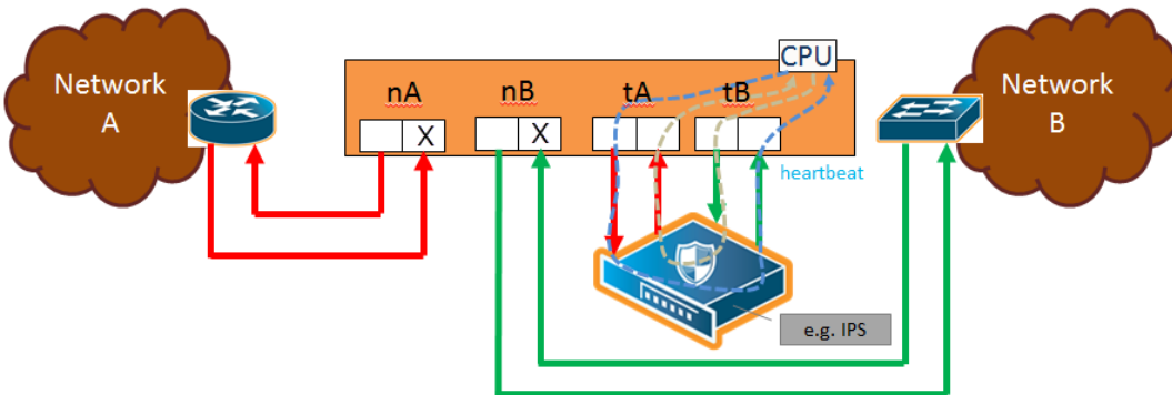
Figure 64 Traffic Path of Drop
